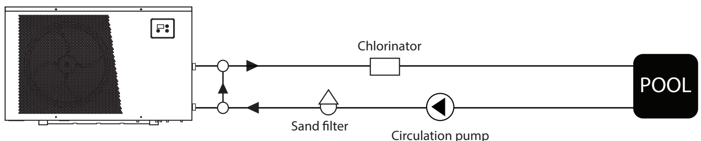
Outline diagram for installation of Q-series
